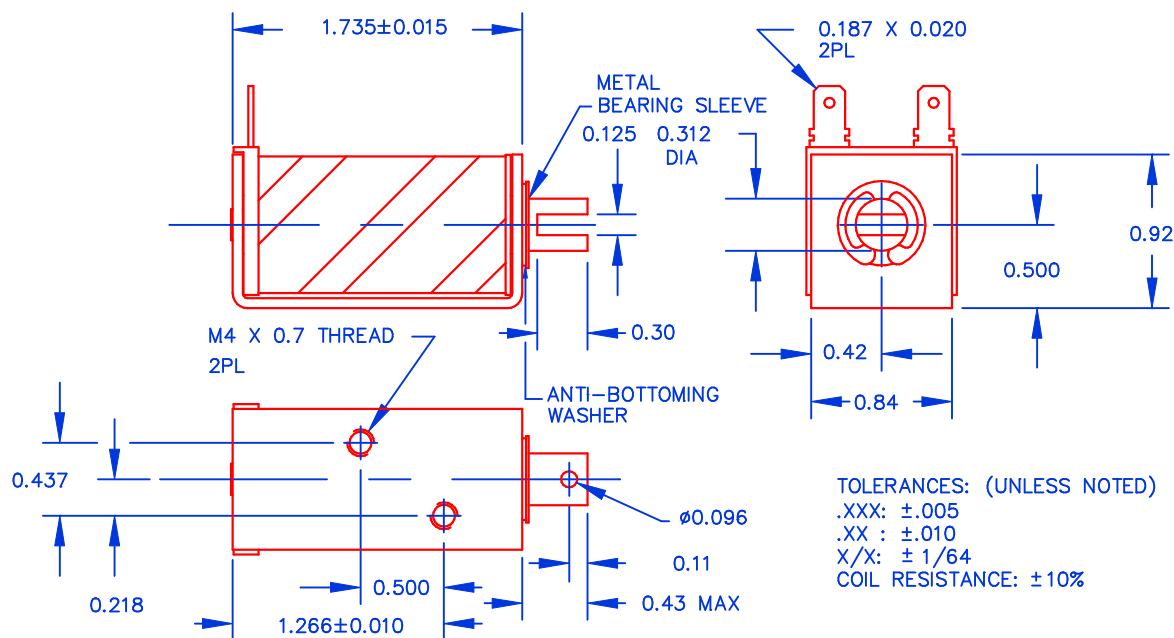
SOLENOID SHOWN ENERGIZED
